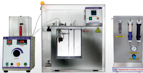
Gassing Tendency Apparatus
